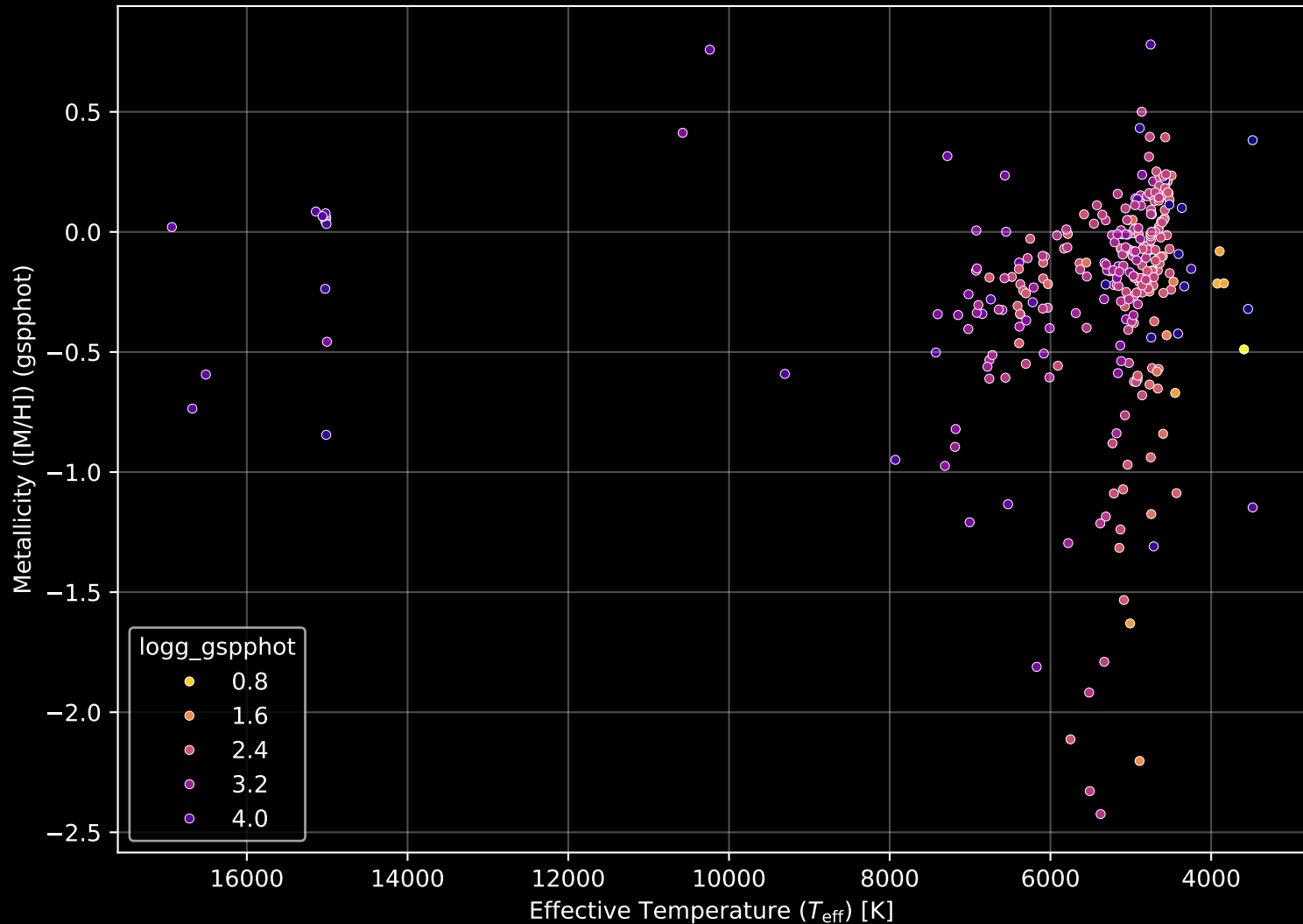
APOGEE DR17 Field: [356+06-C] Stellar Population Parameters (n= 305)
