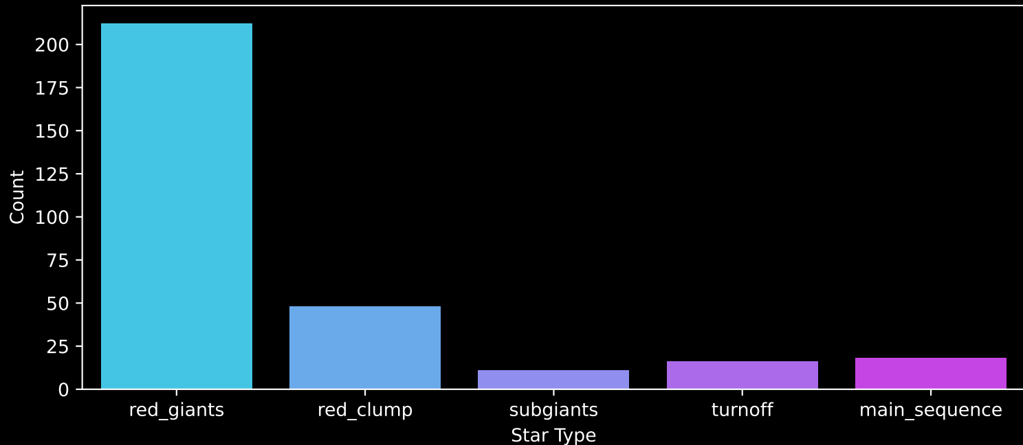
APOGEE DR17 Field: [356+06-C] Count plot of Star Type
