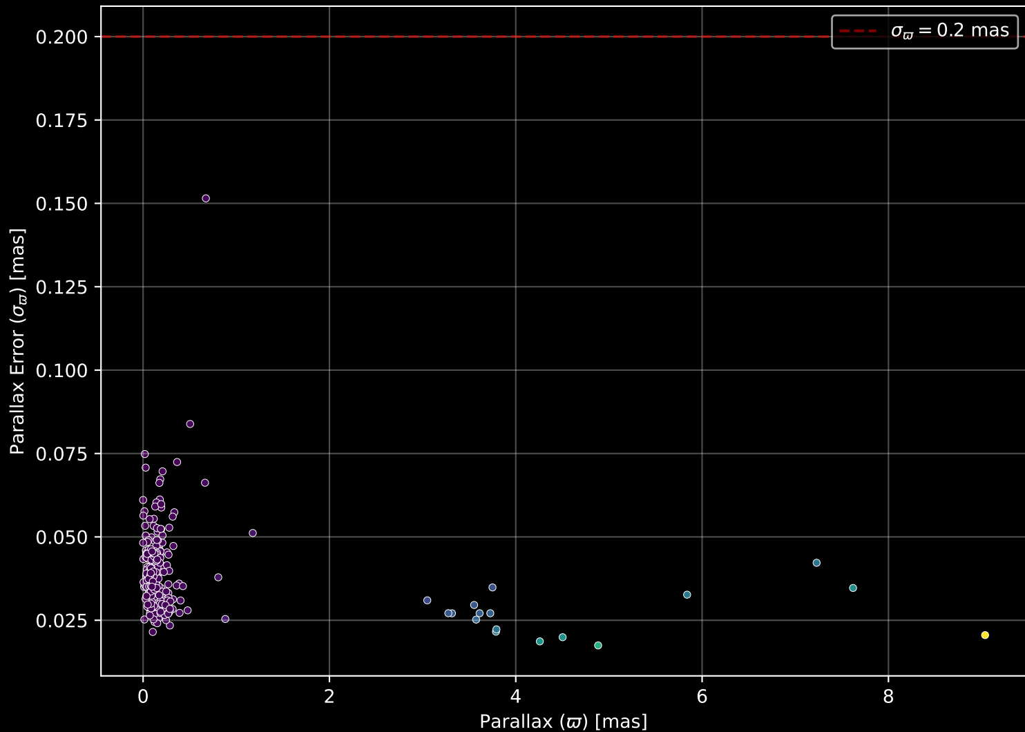
APOGEE DR17 Field: [356+06-C] Parallax Quality (n= 305)
