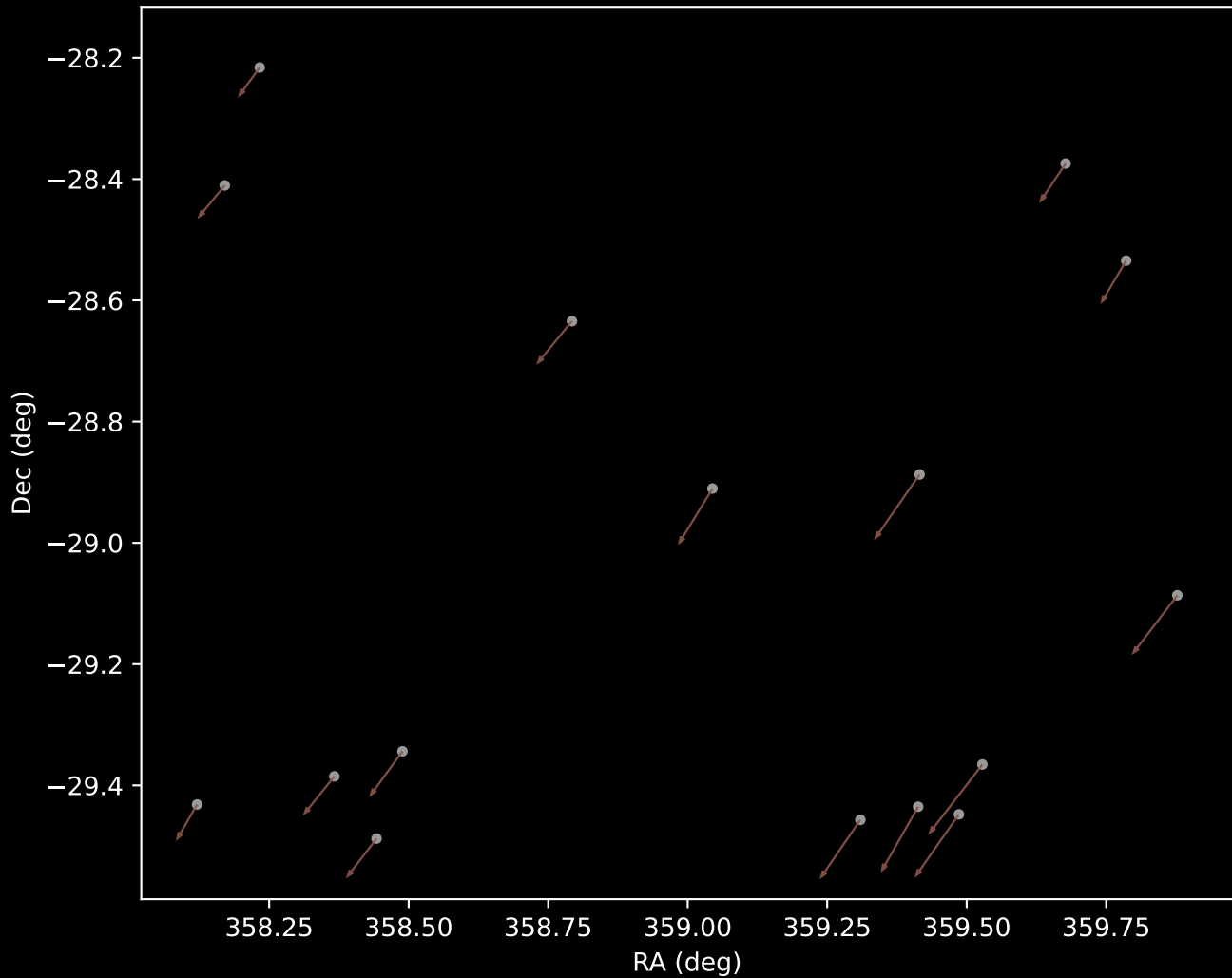
APOGEE DR17 Cluster 10 Proper Motion Vectors (n=16)
