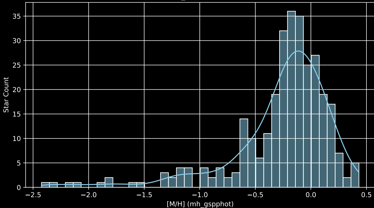
APOGEE DR17 Field: [356+06-C [M/H] (mh_gspphot) (n= 302)
